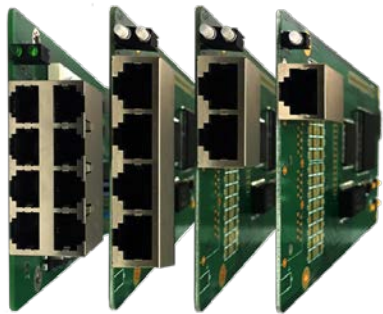
Card boards for FXS, FXO, E1
