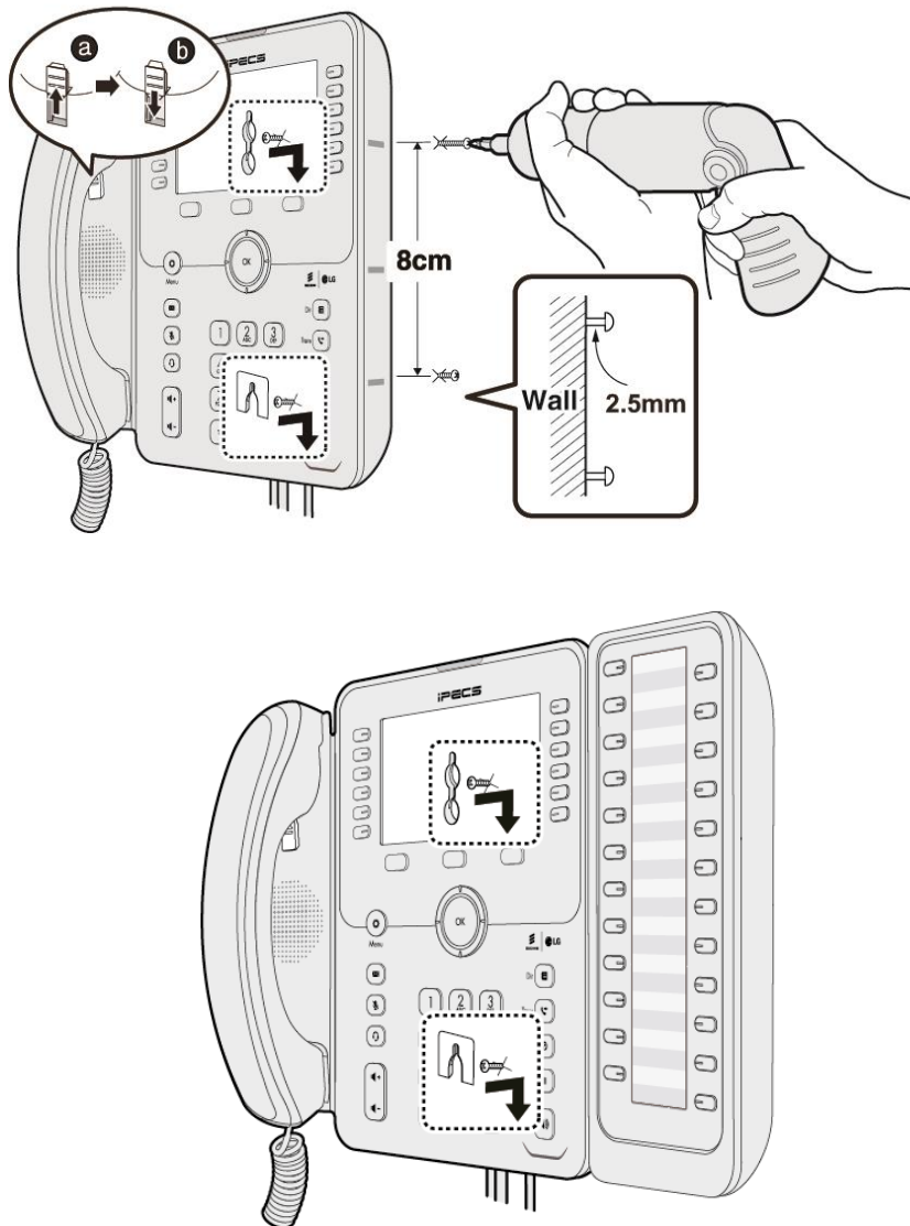
Figure 1.7: Wall Mount
