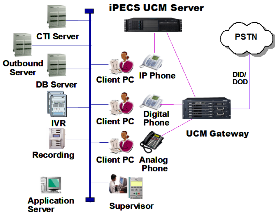
Figure 1 iPECS UCM ACD CTI Basic Configuration
