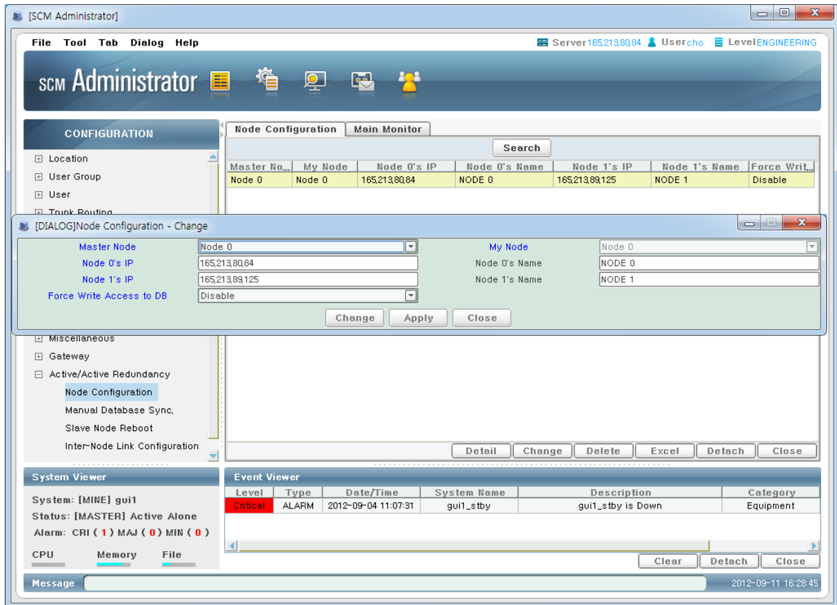
Figure 14. Configuring Node
