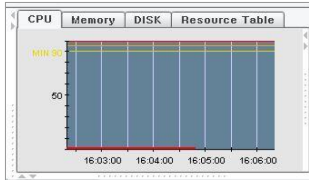
Figure 42. Managing Performance
